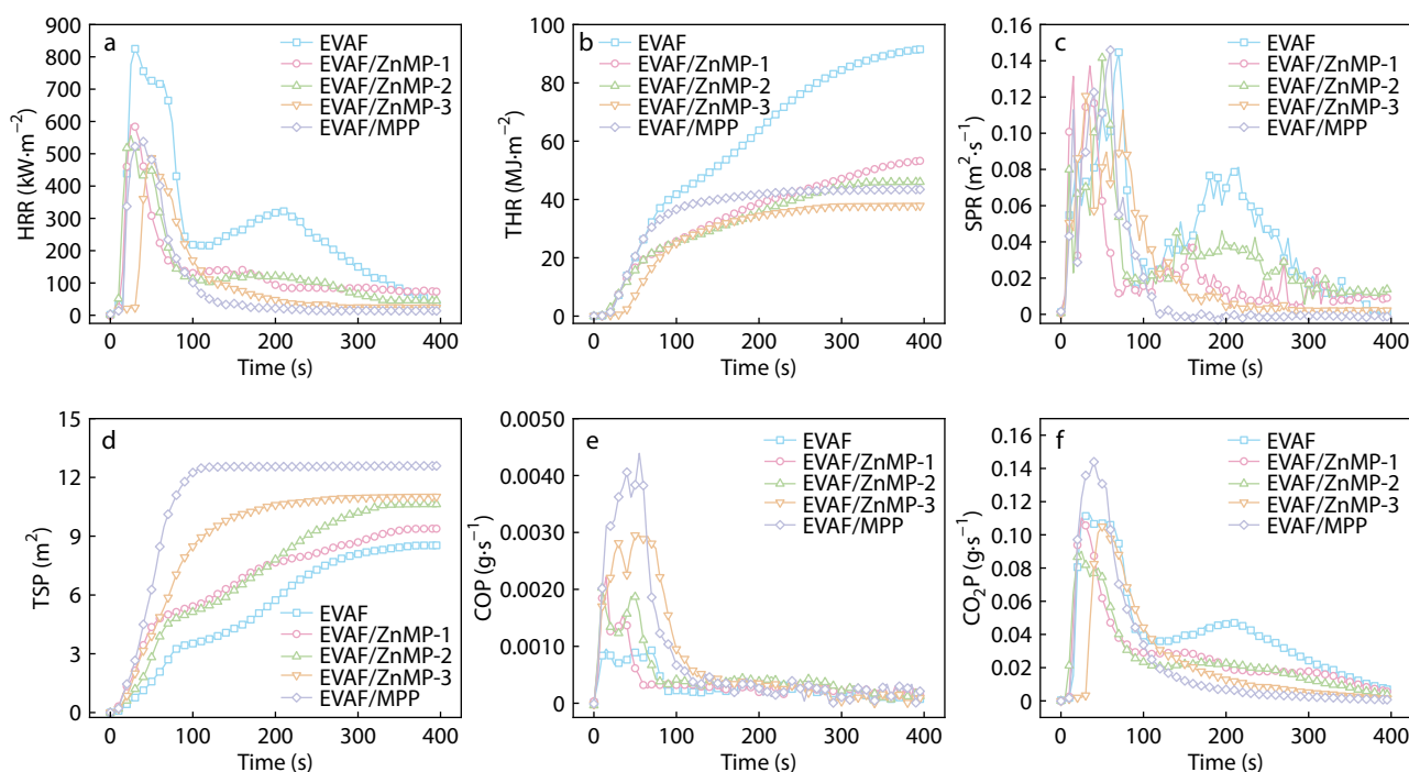
Fig. 10 HRR (a), THR (b), SPR (c), TSP (d), COP (e), and CO 2 P (f) curves of EVAF, EVAF/ZnMP, and EVAF/MPP samples.
